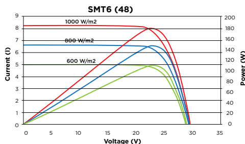
Characteristic IV/Power Curves against Incident Radiation (at 25°C)
